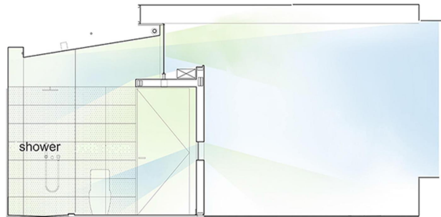
SECTION @ BATHROOM
