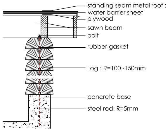
WALL DETAIL
